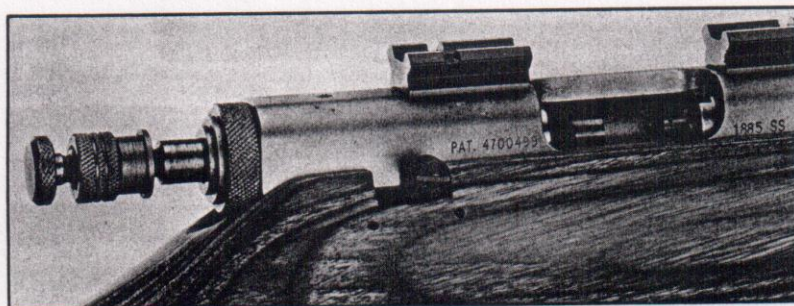
The sliding hammer and its heavy coil spring are retracted by pulling back on the cocking knob until the sear engages. The assembly is retained by the threaded end cap. The side safety blocks the sear and a secondary safety blocks the hammer fall.
